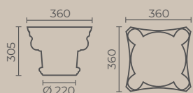
STUB - HS 22R
