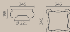
STUB - HS 22K
